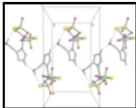
Fig. 2. A view of one-dimensional chains of molecules linked by hydrogen bonds along the c axis. All t Bu groups have been omitted for clarity. Hydrogen bonds are indicated with dashed lines.
